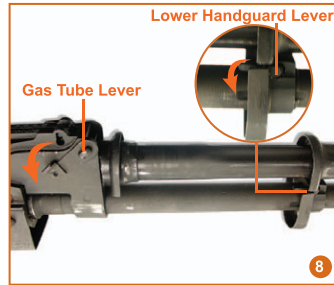
8. Lock the Lower Handguard Lever on the Lower Front Cap. Replace the gas tube and lock it down by turning the Gas Tube Lever back and downward.
