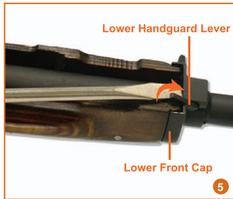
5. Unlock the Lower Handguard Lever on the Lower Front Cap.
